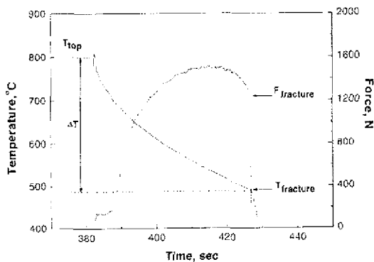
Fig. 18 Temperature and load variation with time
