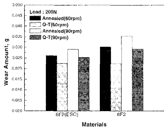
Fig. 16 Wear amount at different velocities
