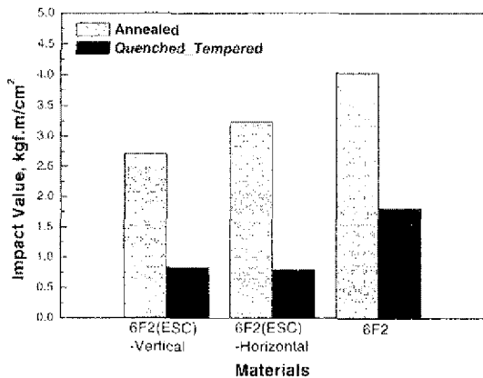
Fig. 15 Comparison of impact values at room temperature
