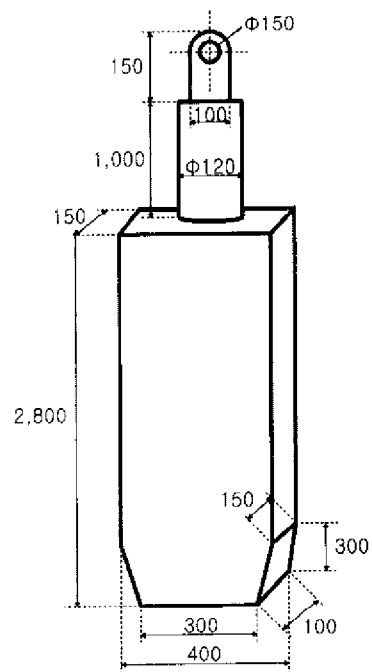
Fig. 2 Schematic drawing of consumable electrode (units of mm)
