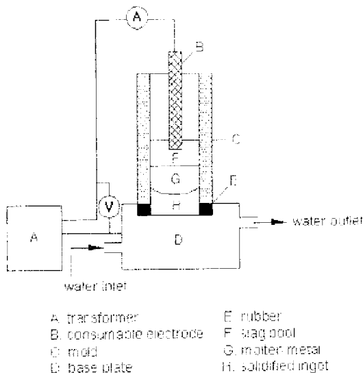
Fig. 1 Schematic drawing of electro-slag casting (ESC) process
