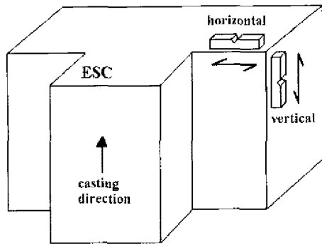
Fig. 5 Impact specimen direction in ESC ingot
