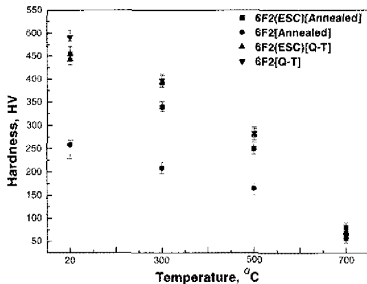
Fig. 14 Hardness values at elevated temperatures
