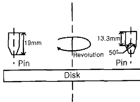
Fig. 6 Schematic drawing of pin-on-disk test apparatus
