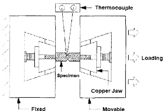
Fig. 10 Schematic drawing of loading mechanism in the Gleeble test machine
